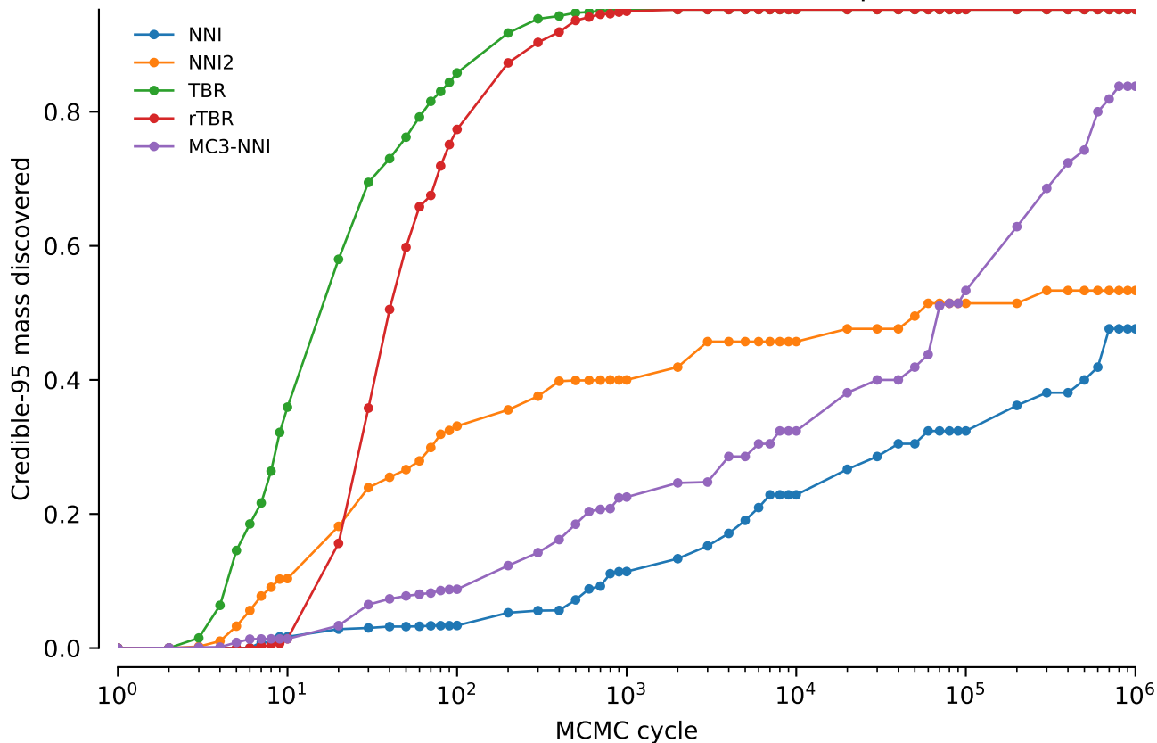
vert.nd4l.tw0: Credible-95 mass discovered: power = 0.4
