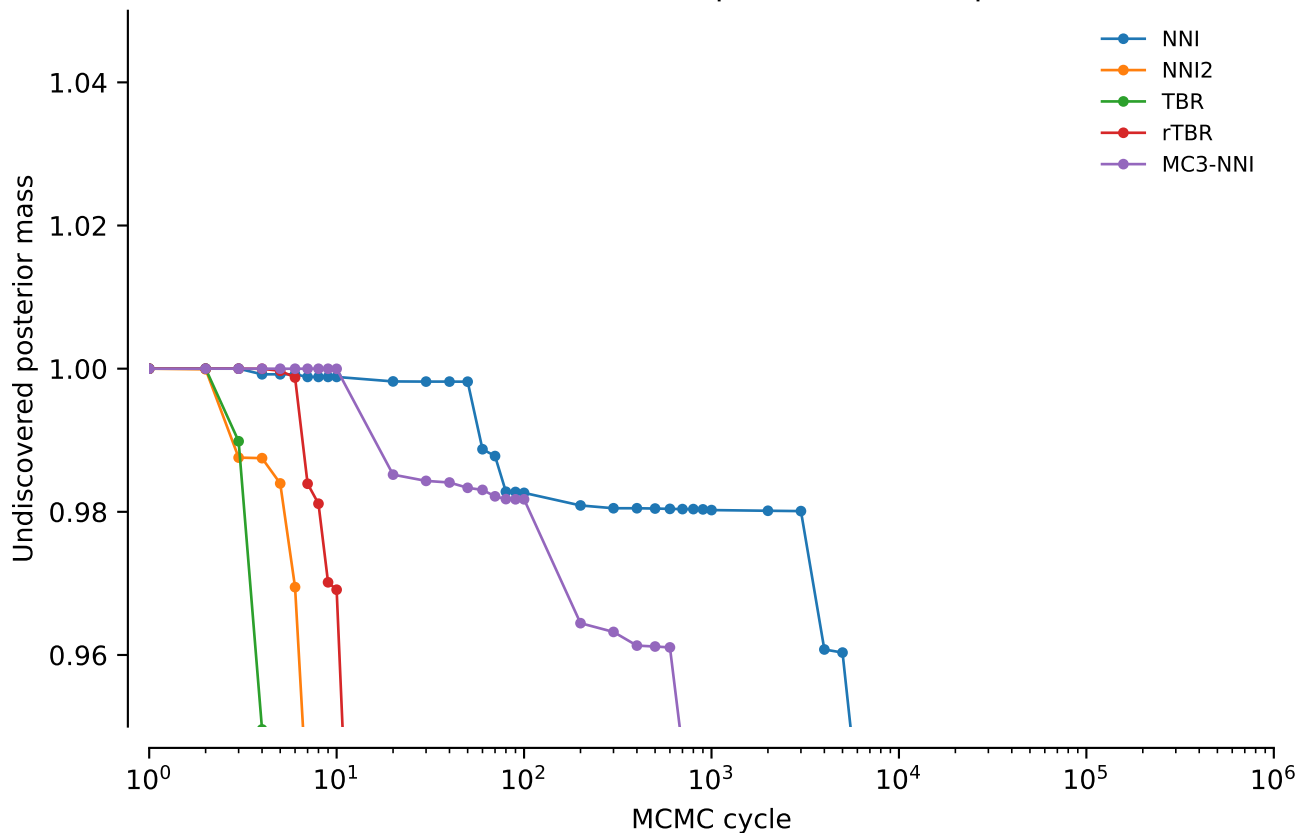
vert.nd4l.tw0: Undiscovered posterior mass: power = 0.5
