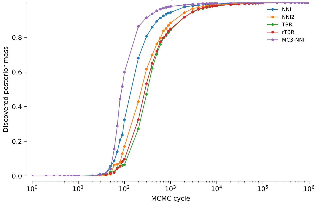
vert.nd4l.tw0: Discovered posterior mass: power = 0
