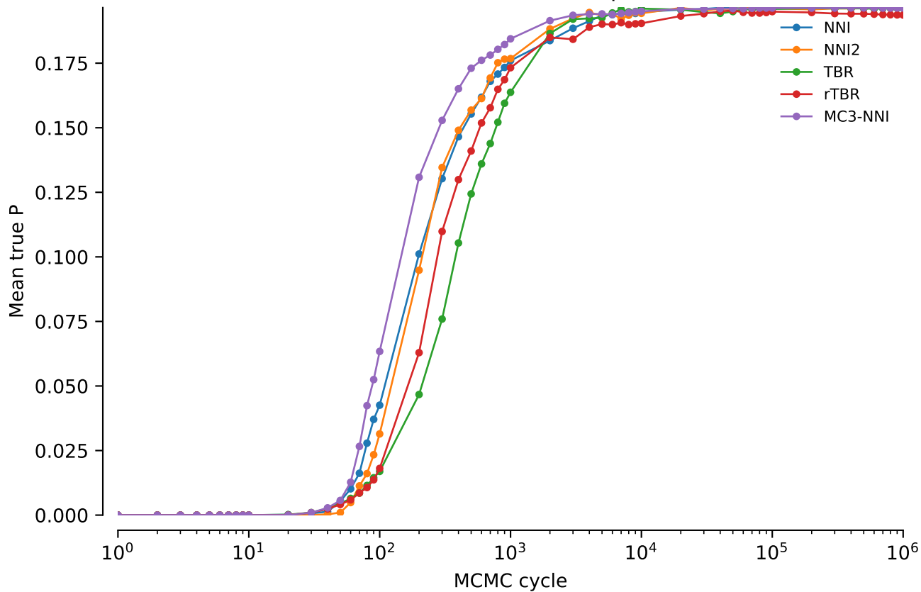
vert.nd4l.tw0: Mean true P: power = 0
