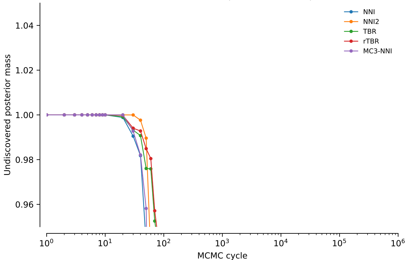
vert.nd4l.tw0: Undiscovered posterior mass: power = 0
