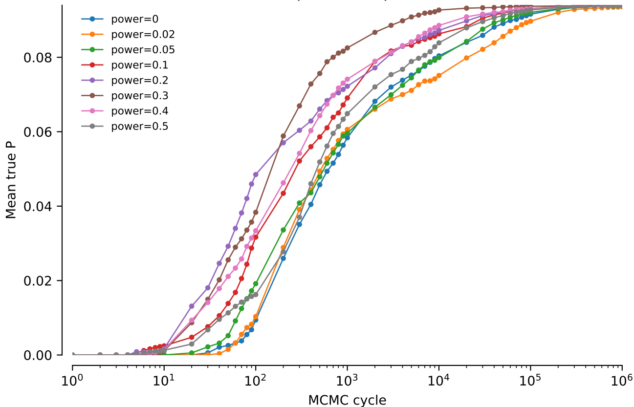
vert.nd4l.tw5: NNI power comparison: Mean true P
