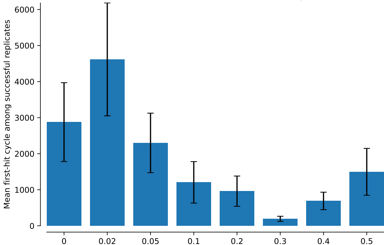
vert.nd4l.tw5: NNI: mean MAP first-hit cycle
