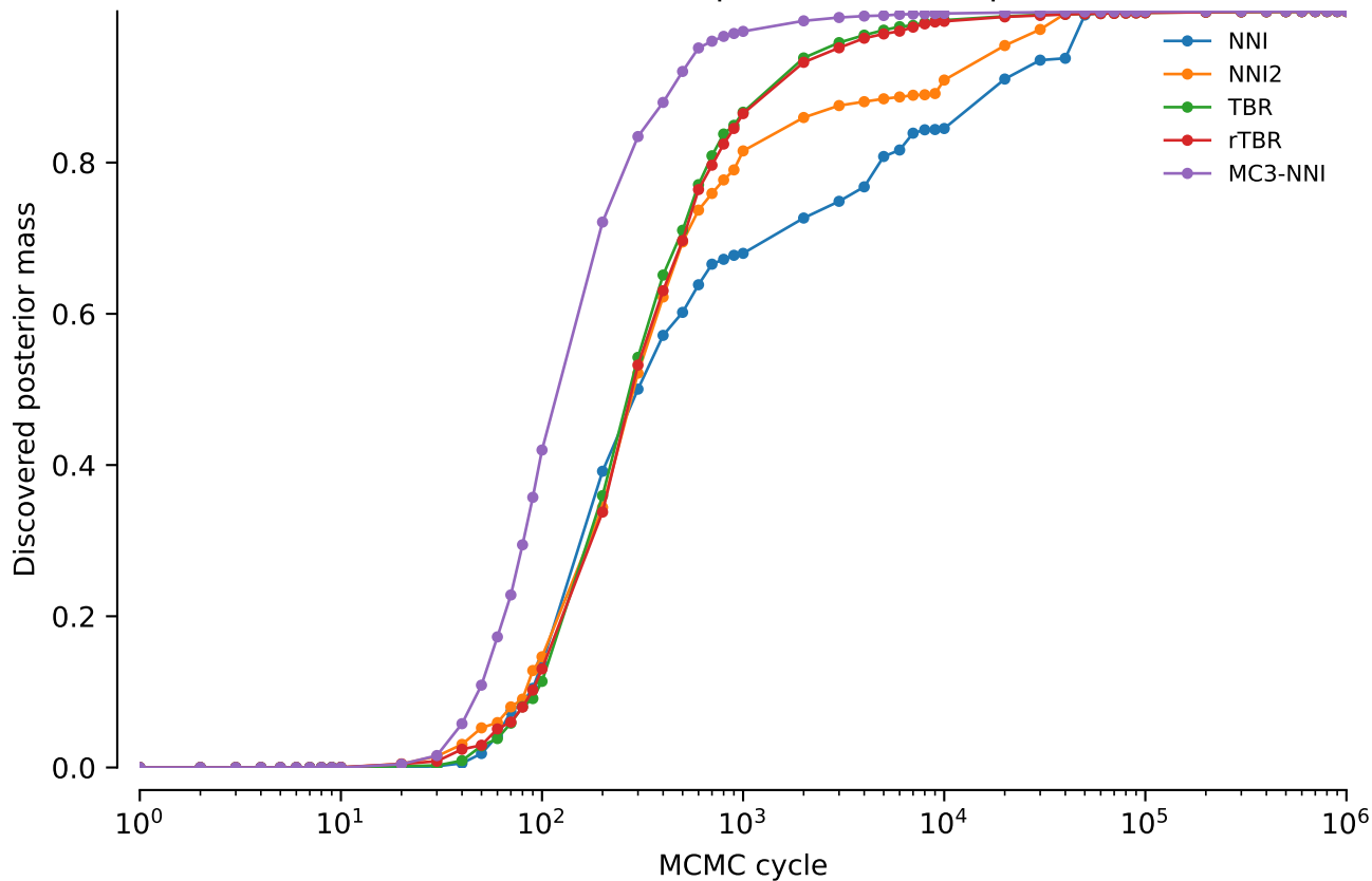
vert.nd4l.tw5: Discovered posterior mass: power = 0.02
