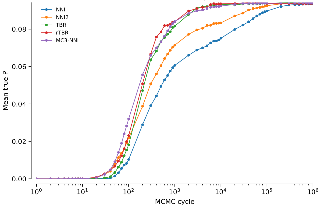
vert.nd4l.tw5: Mean true P: power = 0.02
