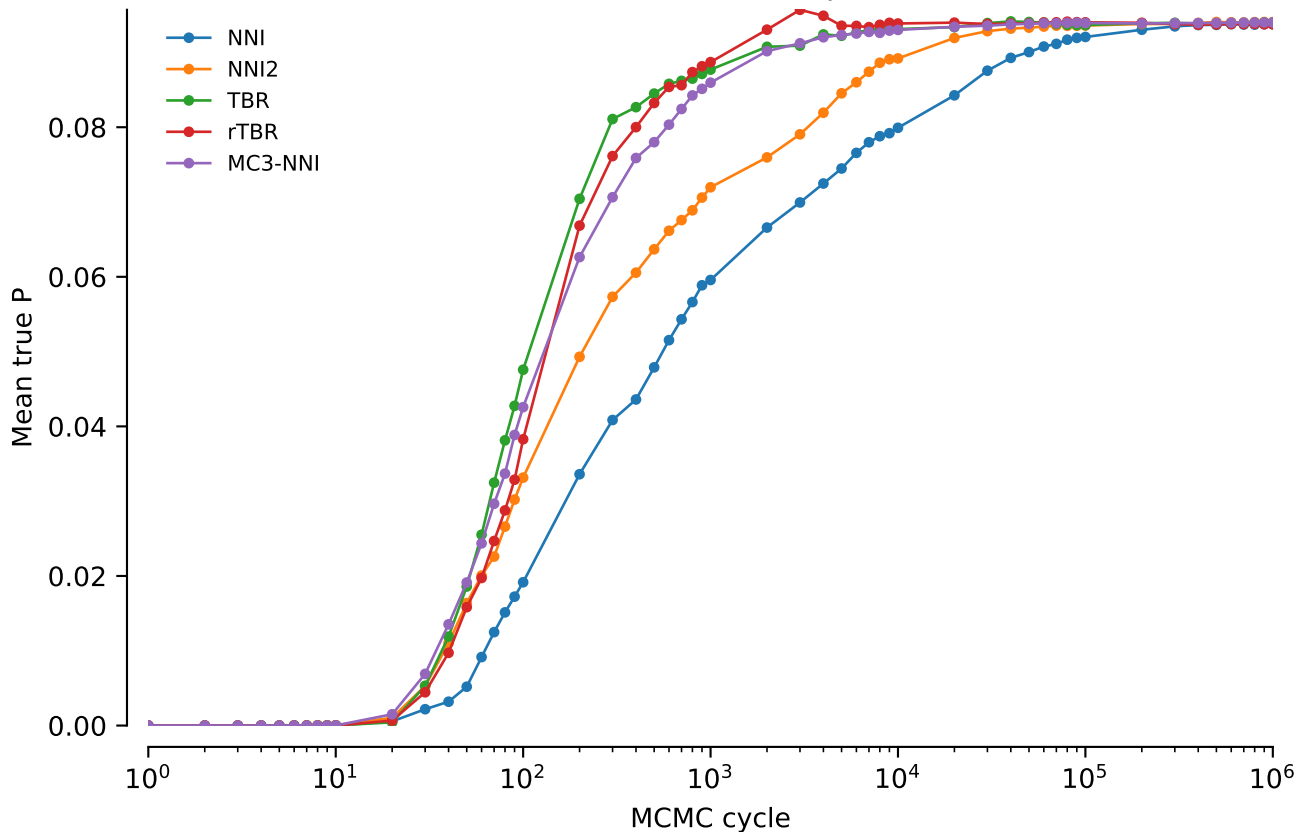
vert.nd4l.tw5: Mean true P: power = 0.05
