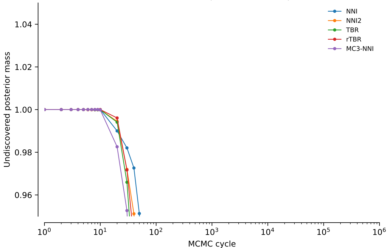
vert.nd4l.tw5: Undiscovered posterior mass: power = 0.05
