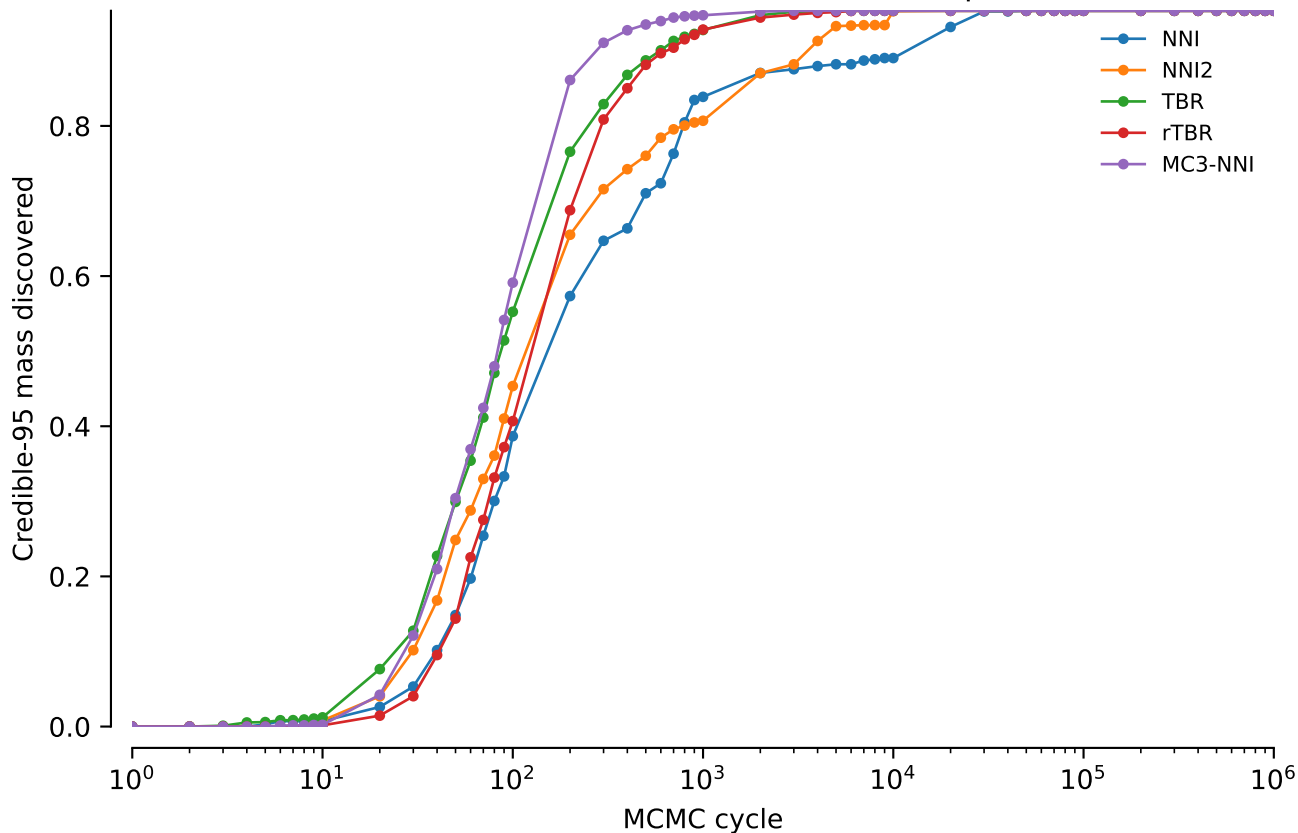
vert.nd4l.tw5: Credible-95 mass discovered: power = 0.1
