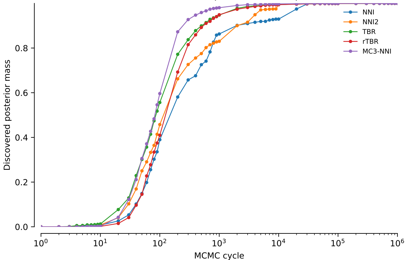
vert.nd4l.tw5: Discovered posterior mass: power = 0.1
