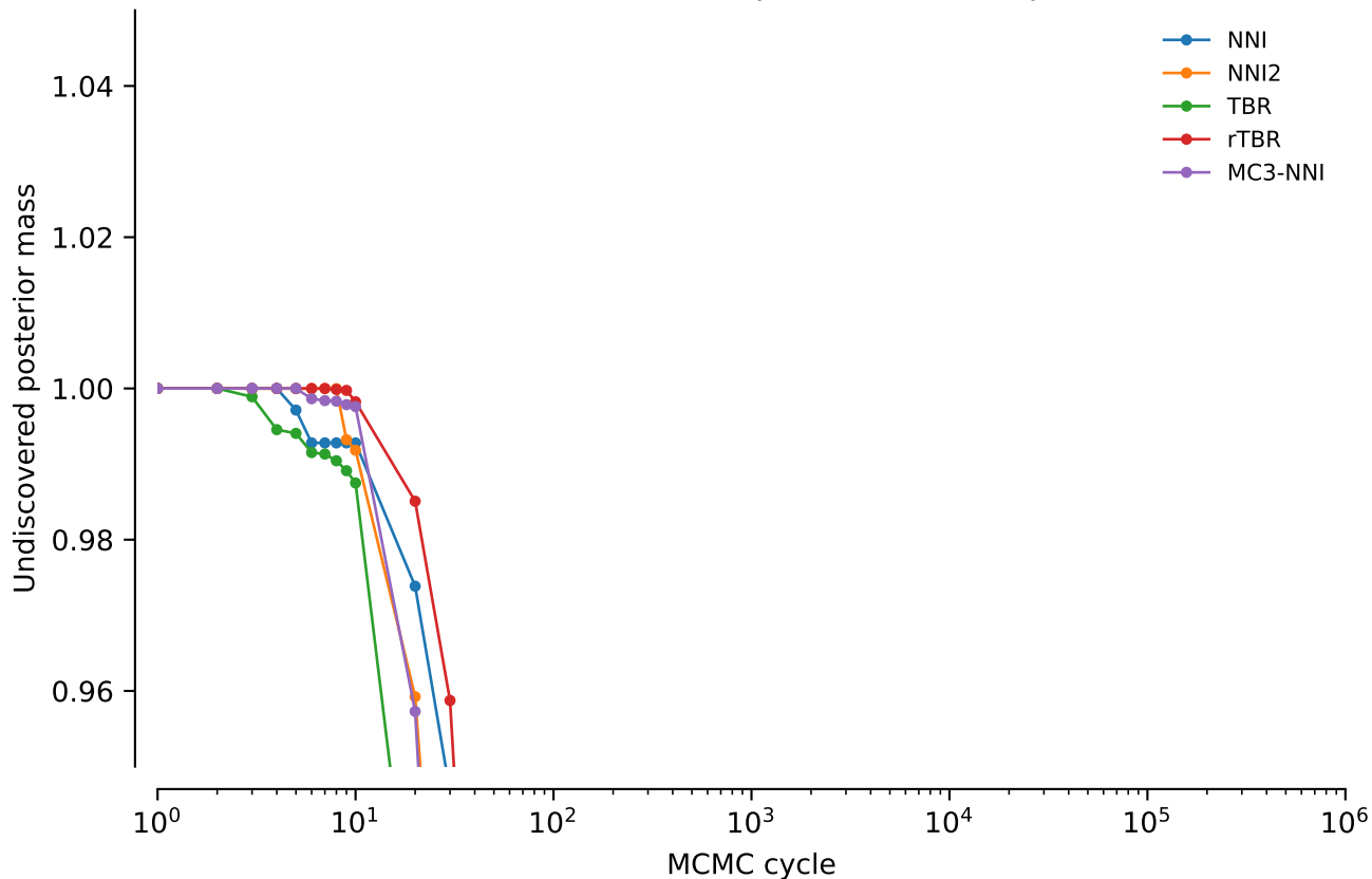
vert.nd4l.tw5: Undiscovered posterior mass: power = 0.1
