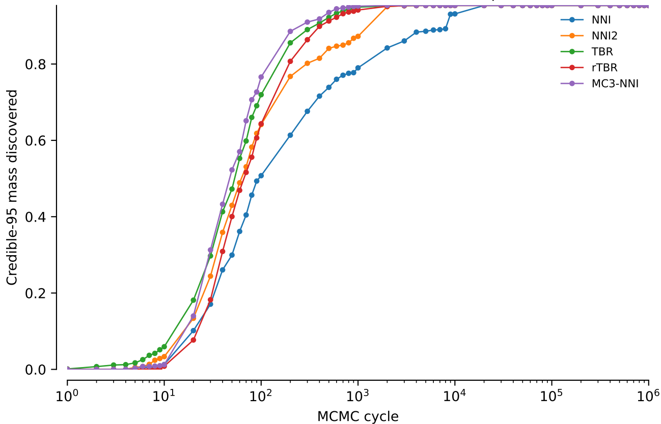
vert.nd4l.tw5: Credible-95 mass discovered: power = 0.2
