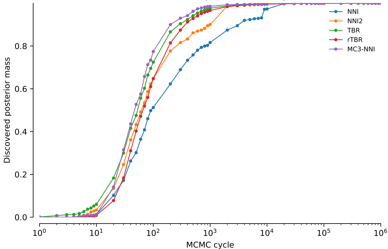
vert.nd4l.tw5: Discovered posterior mass: power = 0.2
