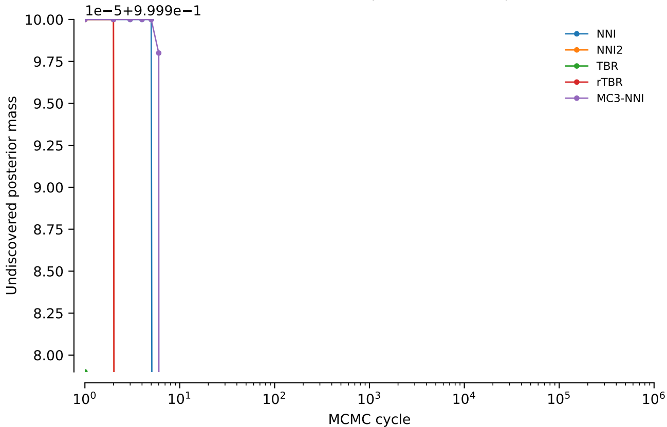
vert.nd4l.tw5: Undiscovered posterior mass: power = 0.3
