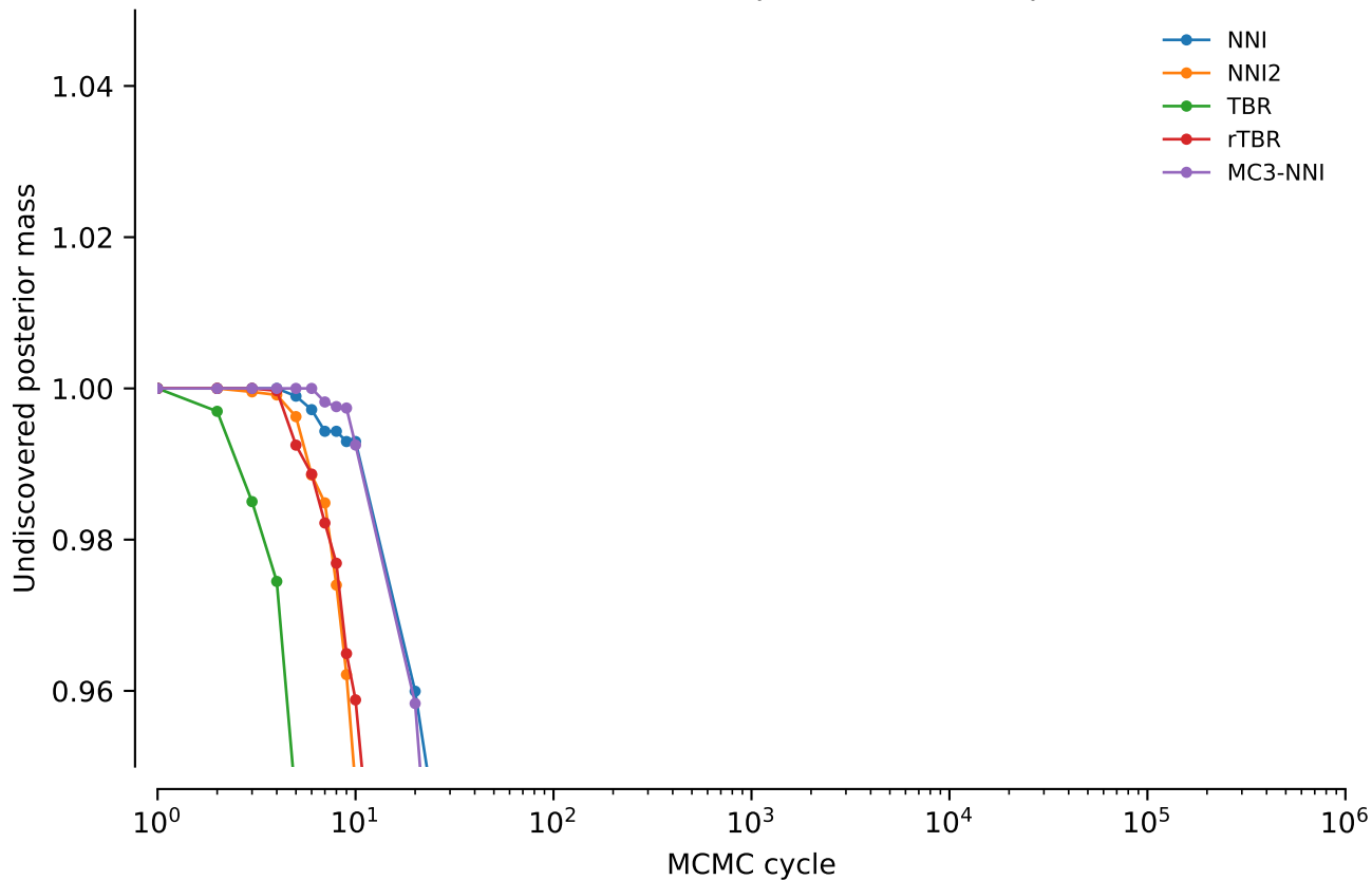
vert.nd4l.tw5: Undiscovered posterior mass: power = 0.5
