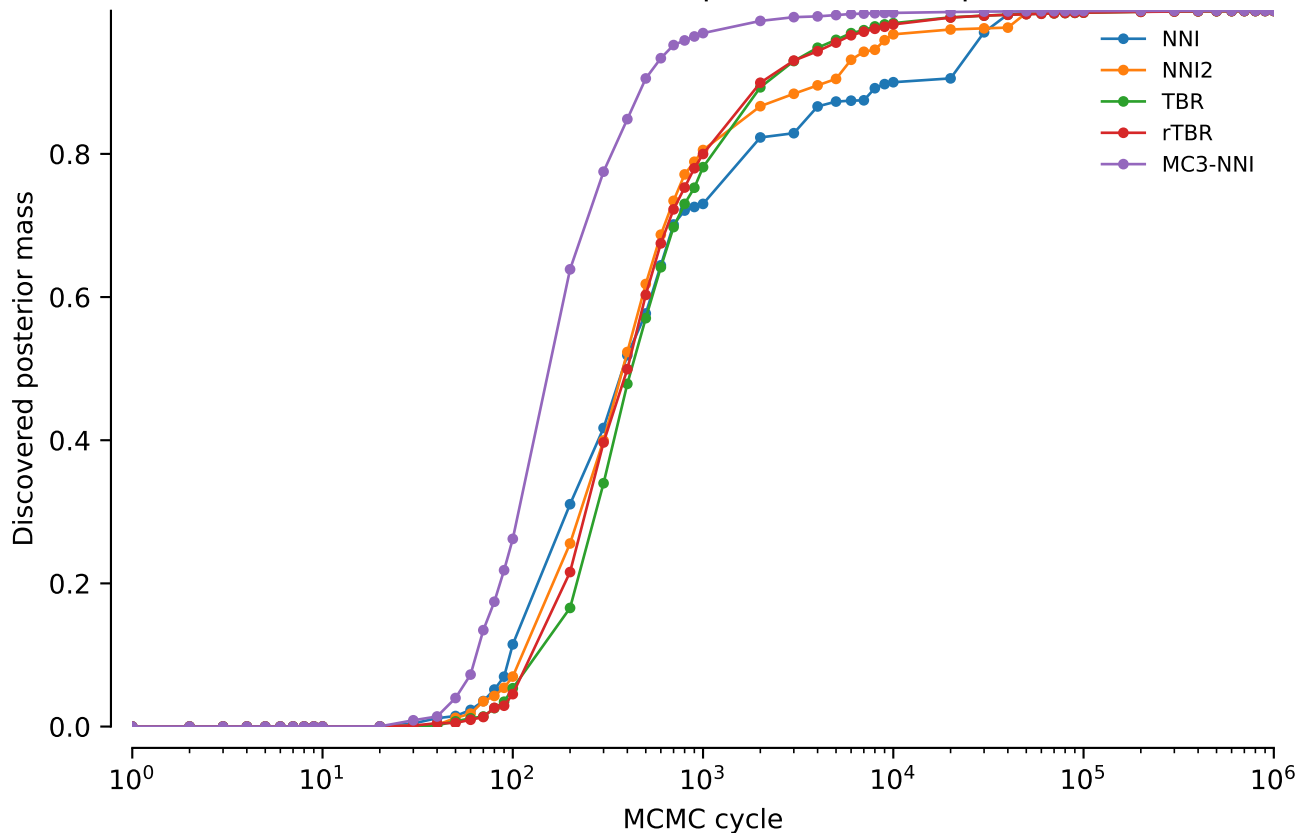
vert.nd4l.tw5: Discovered posterior mass: power = 0
