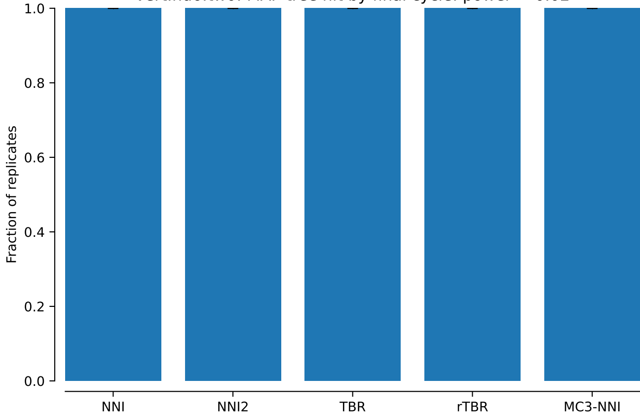
vert.nd6.tw0: MAP tree hit by final cycle: power = 0.02
