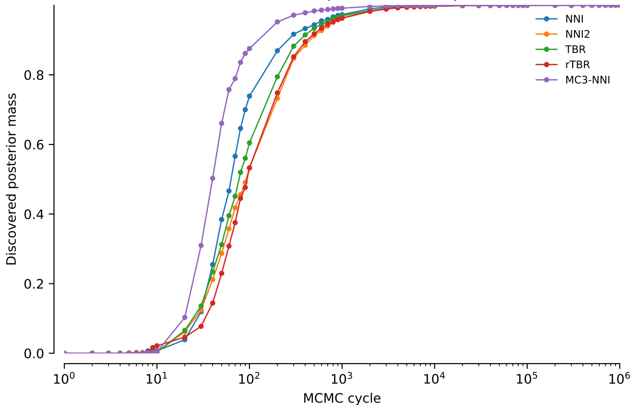
vert.nd6.tw0: Discovered posterior mass: power = 0.02
