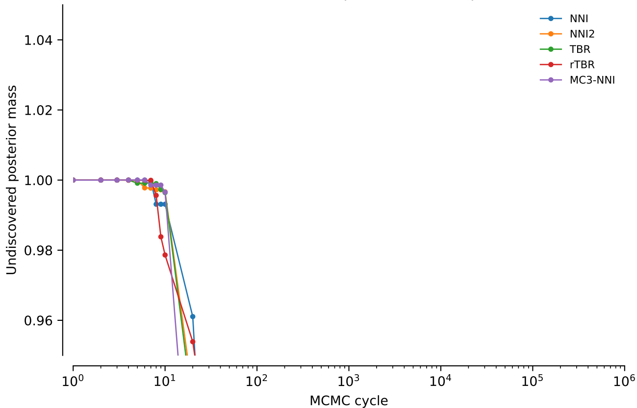
vert.nd6.tw0: Undiscovered posterior mass: power = 0.02
