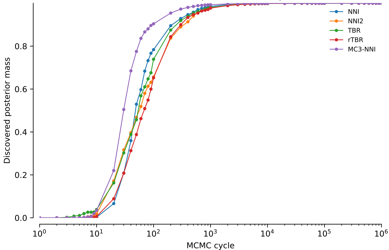
vert.nd6.tw0: Discovered posterior mass: power = 0.05
