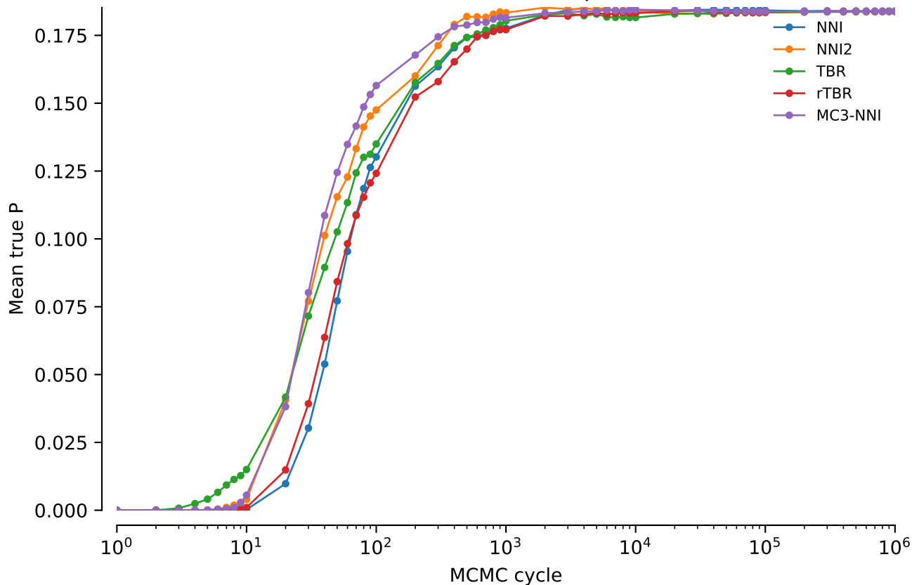
vert.nd6.tw0: Mean true P: power = 0.05
