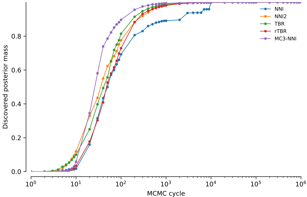
vert.nd6.tw0: Discovered posterior mass: power = 0.1
