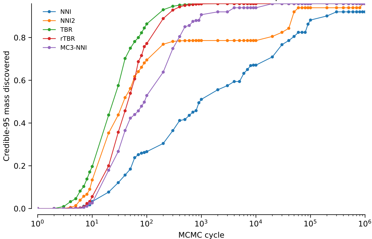
vert.nd6.tw0: Credible-95 mass discovered: power = 0.2
