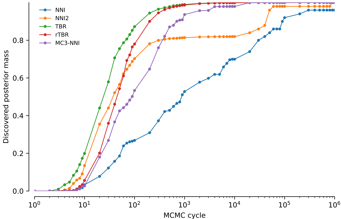
vert.nd6.tw0: Discovered posterior mass: power = 0.2
