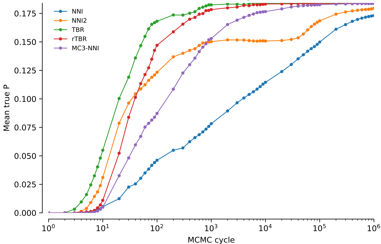
vert.nd6.tw0: Mean true P: power = 0.2
