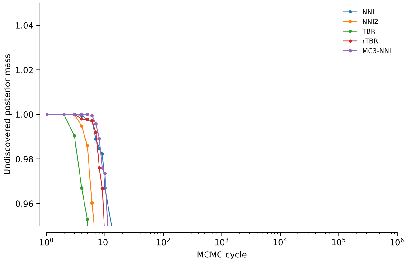
vert.nd6.tw0: Undiscovered posterior mass: power = 0.2
