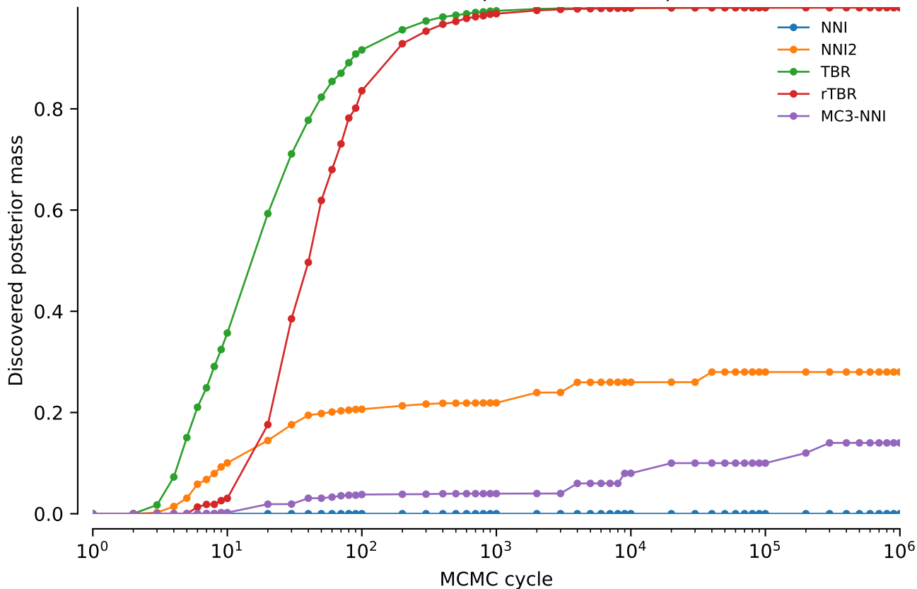
vert.nd6.tw0: Discovered posterior mass: power = 0.4
