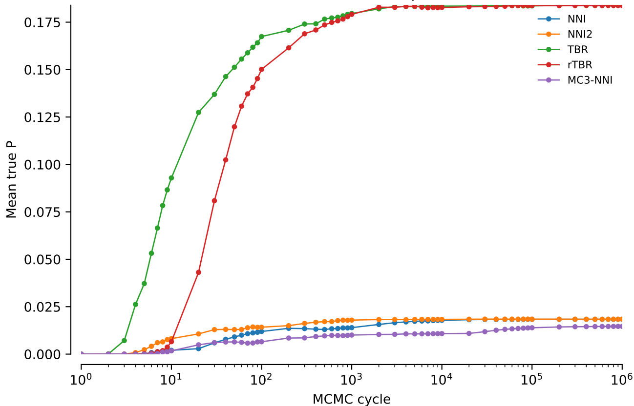
vert.nd6.tw0: Mean true P: power = 0.5
