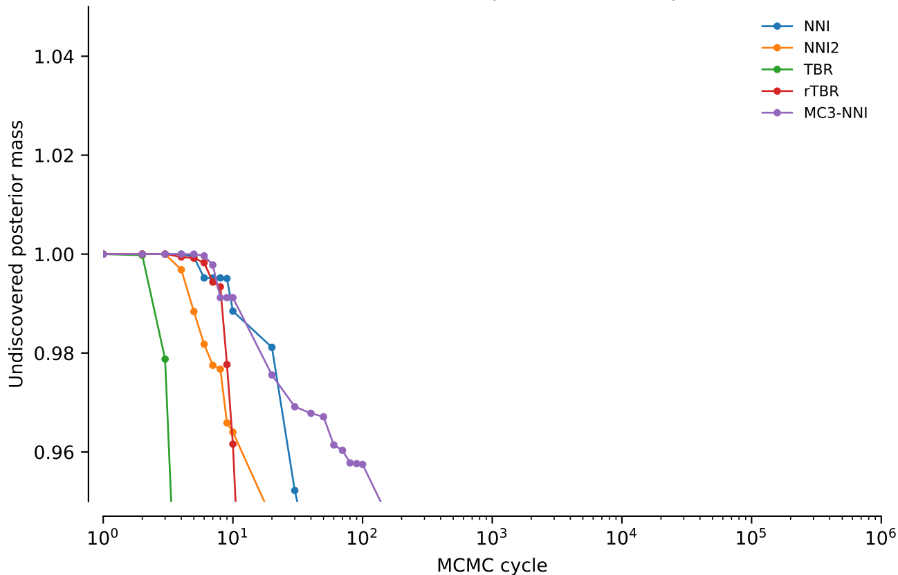
vert.nd6.tw0: Undiscovered posterior mass: power = 0.5
