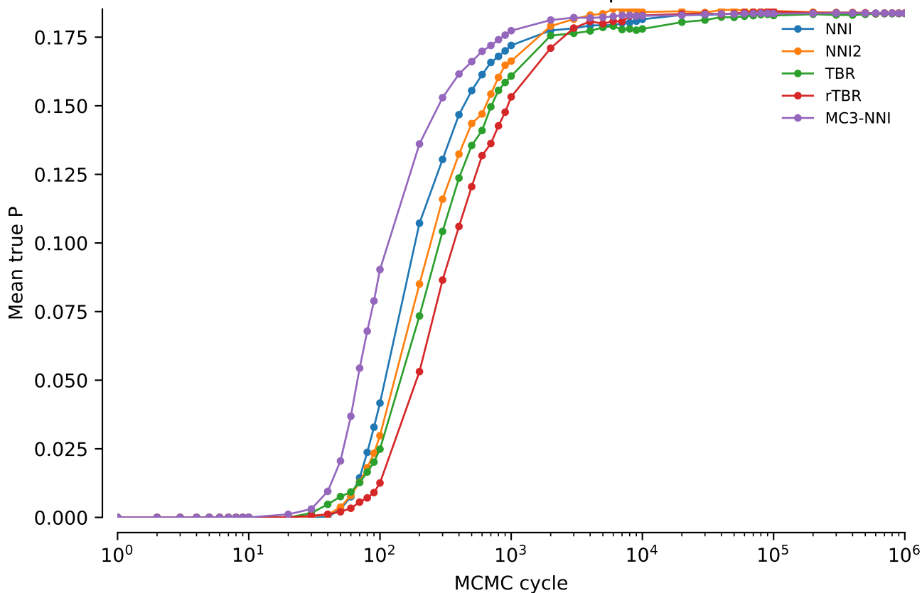
vert.nd6.tw0: Mean true P: power = 0
