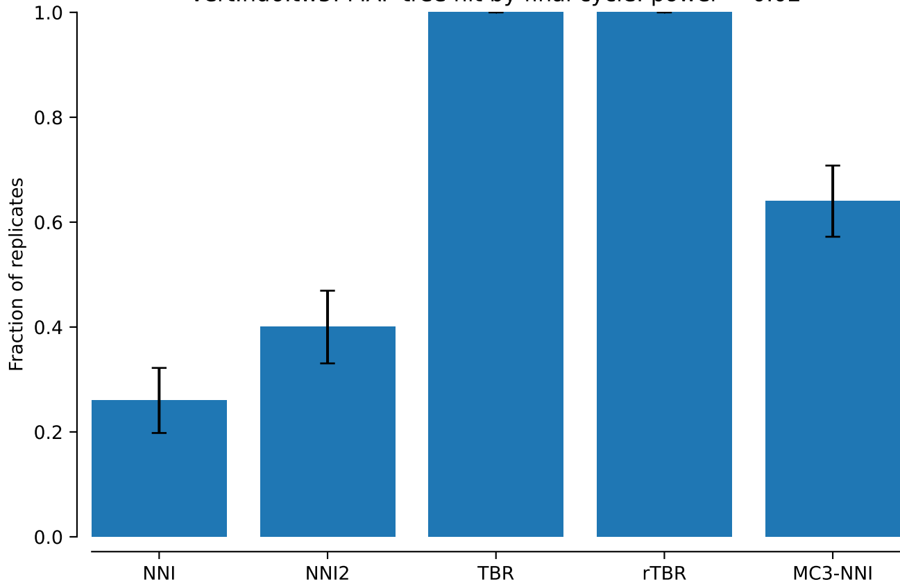
vert.nd6.tw5: MAP tree hit by final cycle: power = 0.02
