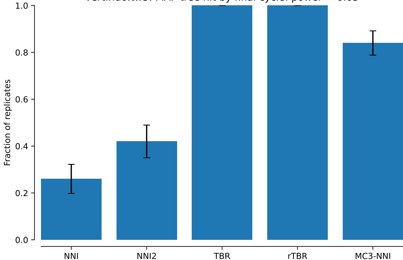
vert.nd6.tw5: MAP tree hit by final cycle: power = 0.05
