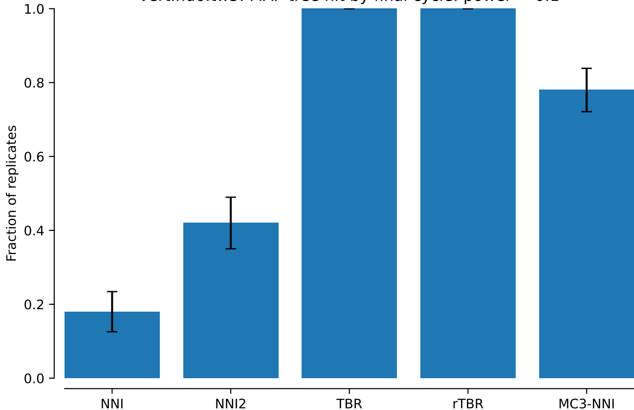
vert.nd6.tw5: MAP tree hit by final cycle: power = 0.1
