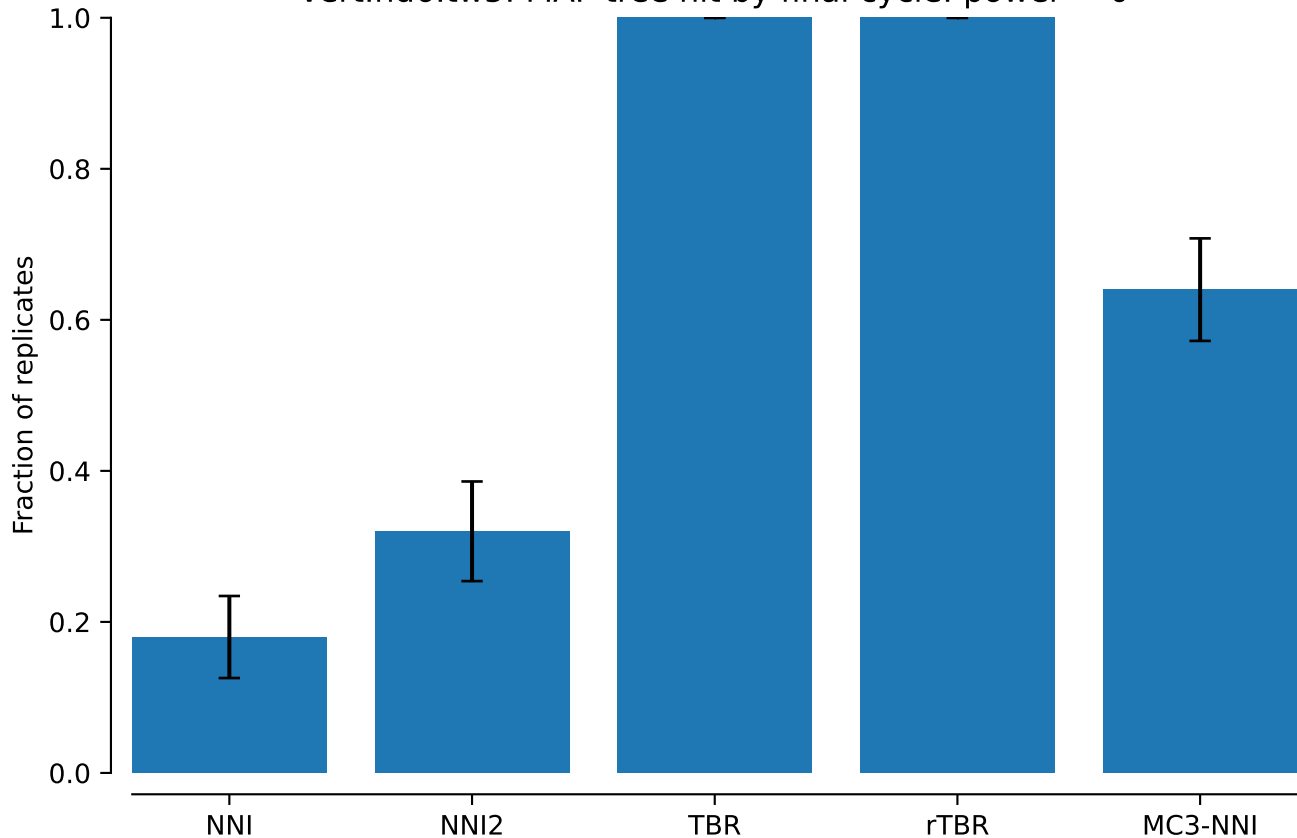
vert.nd6.tw5: MAP tree hit by final cycle: power = 0
