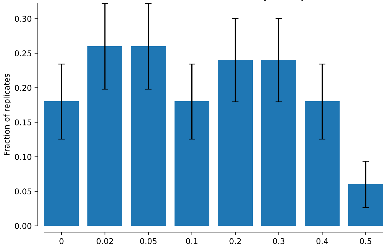
vert.nd6.tw5: NNI: MAP tree hit by final cycle
