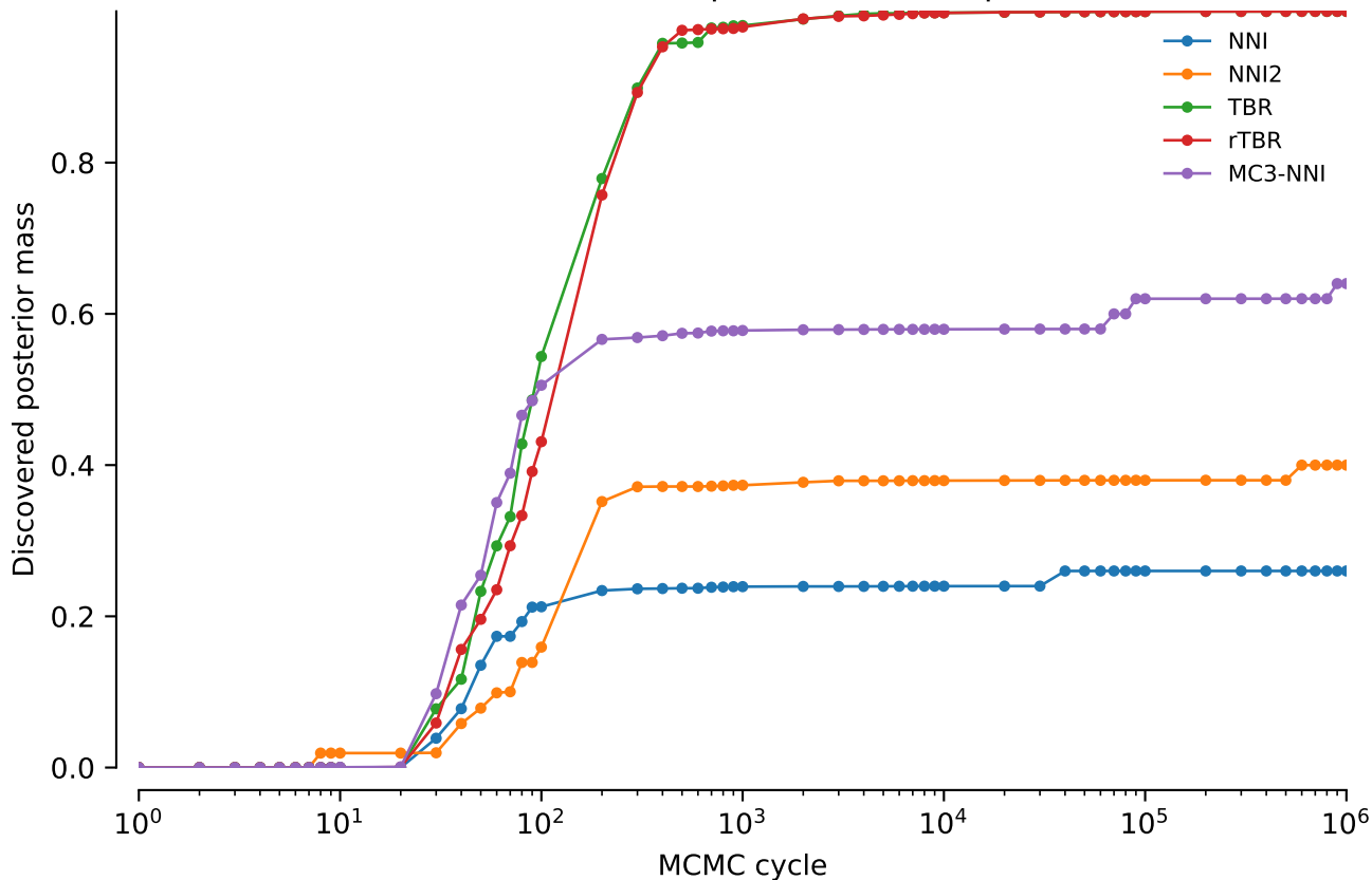
vert.nd6.tw5: Discovered posterior mass: power = 0.02
