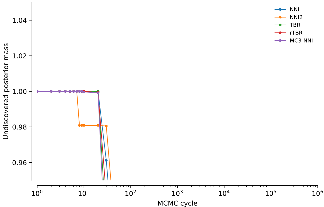
vert.nd6.tw5: Undiscovered posterior mass: power = 0.02
