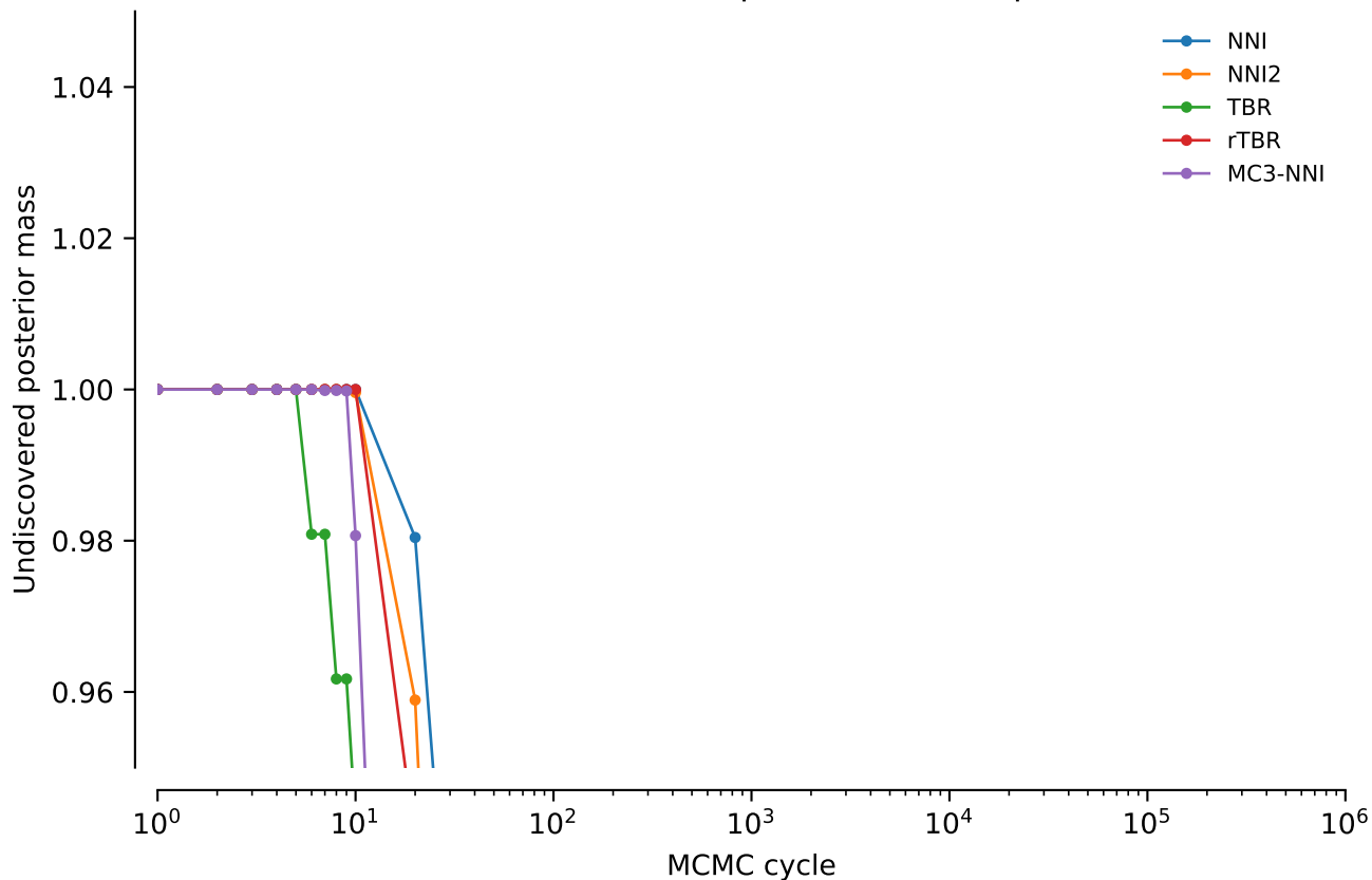
vert.nd6.tw5: Undiscovered posterior mass: power = 0.05
