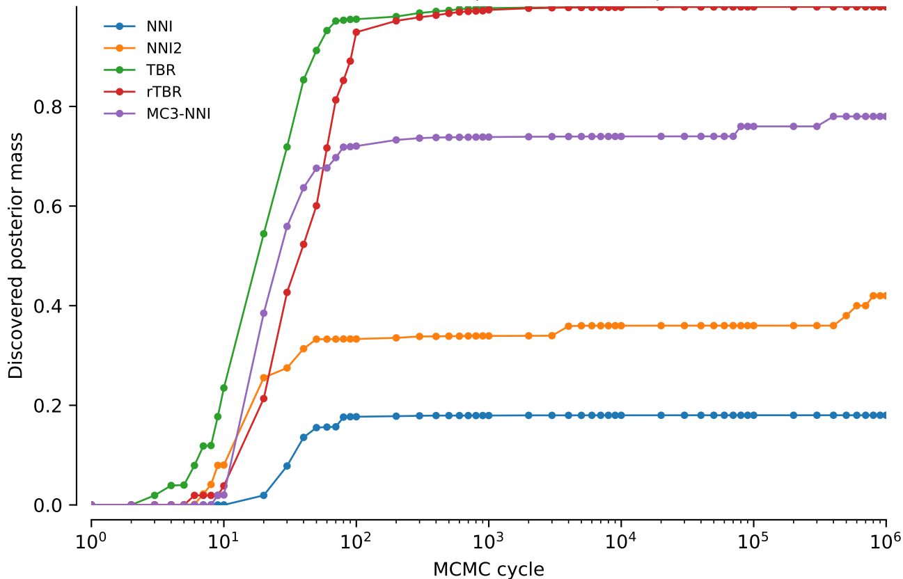
vert.nd6.tw5: Discovered posterior mass: power = 0.1
