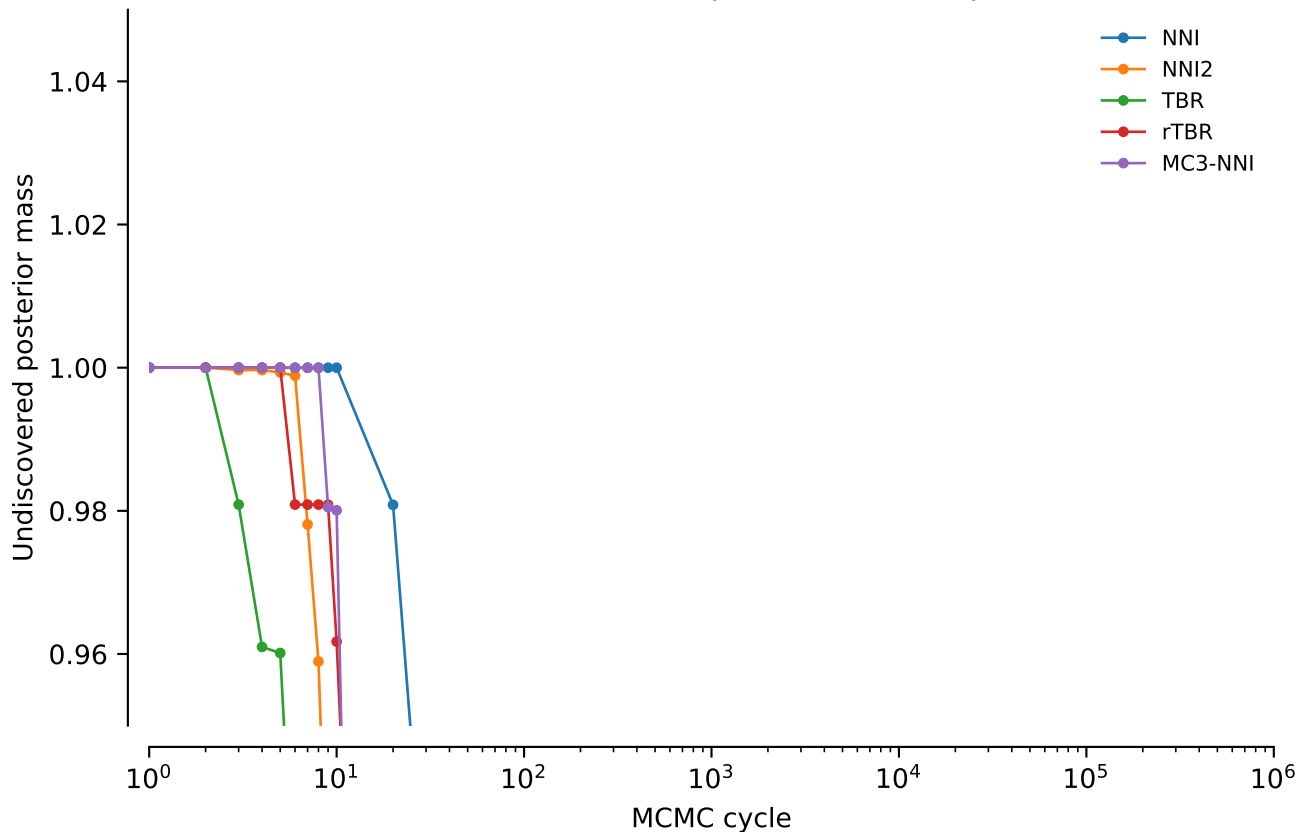
vert.nd6.tw5: Undiscovered posterior mass: power = 0.1
