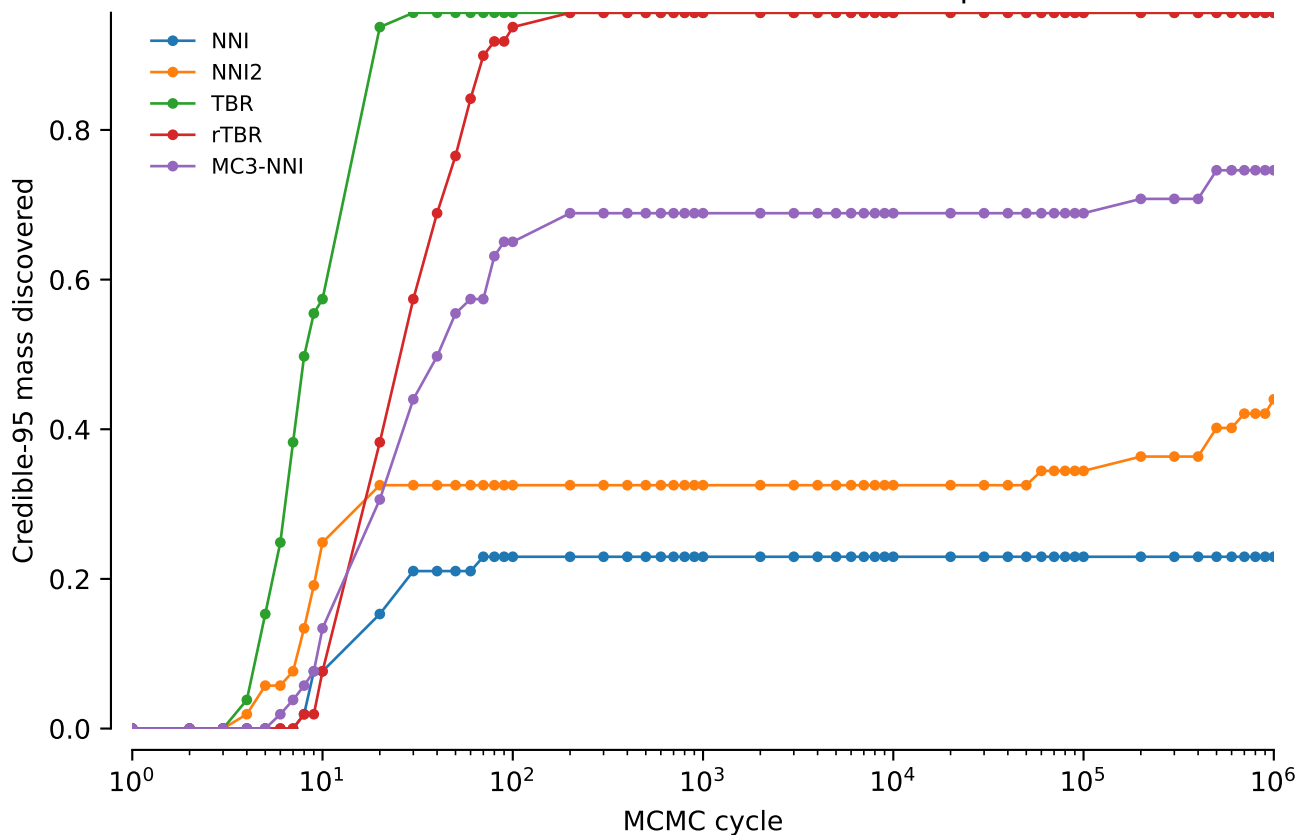
vert.nd6.tw5: Credible-95 mass discovered: power = 0.2
