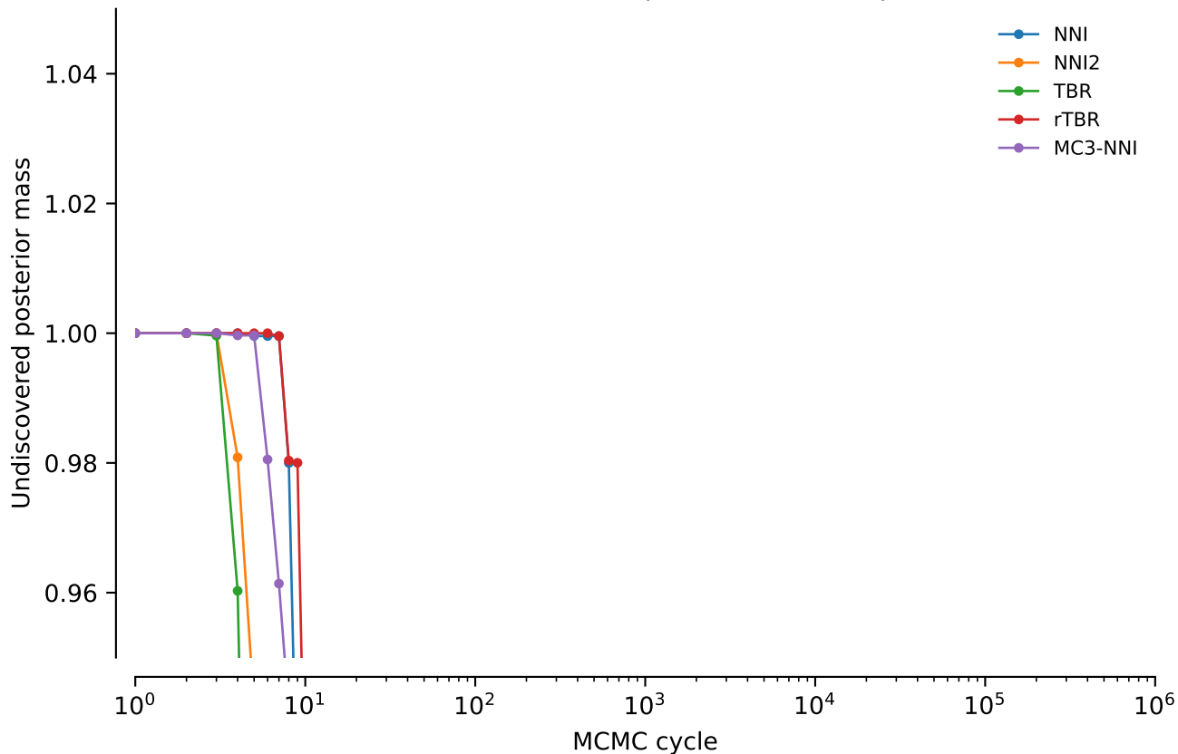
vert.nd6.tw5: Undiscovered posterior mass: power = 0.2
