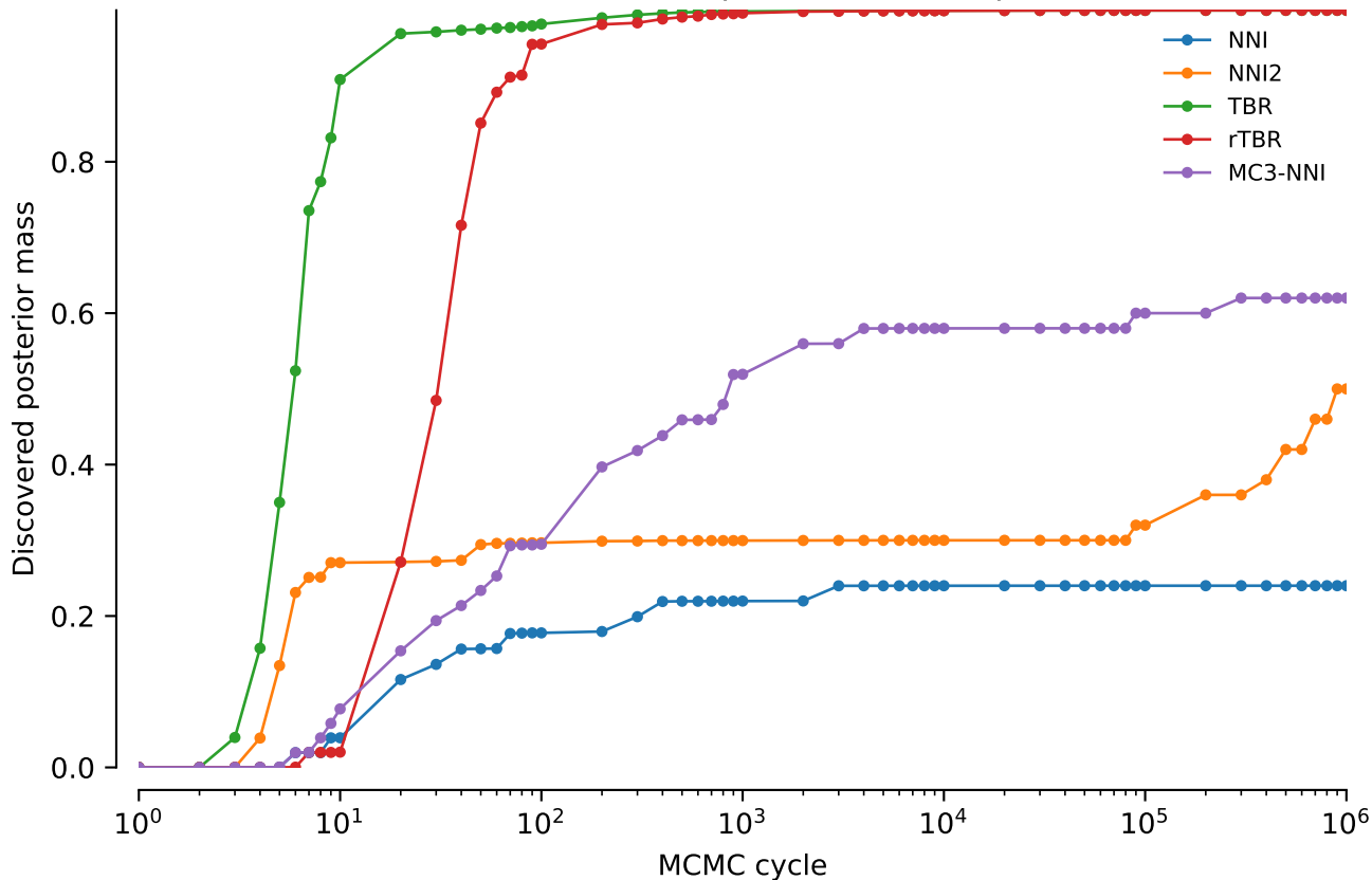
vert.nd6.tw5: Discovered posterior mass: power = 0.3
