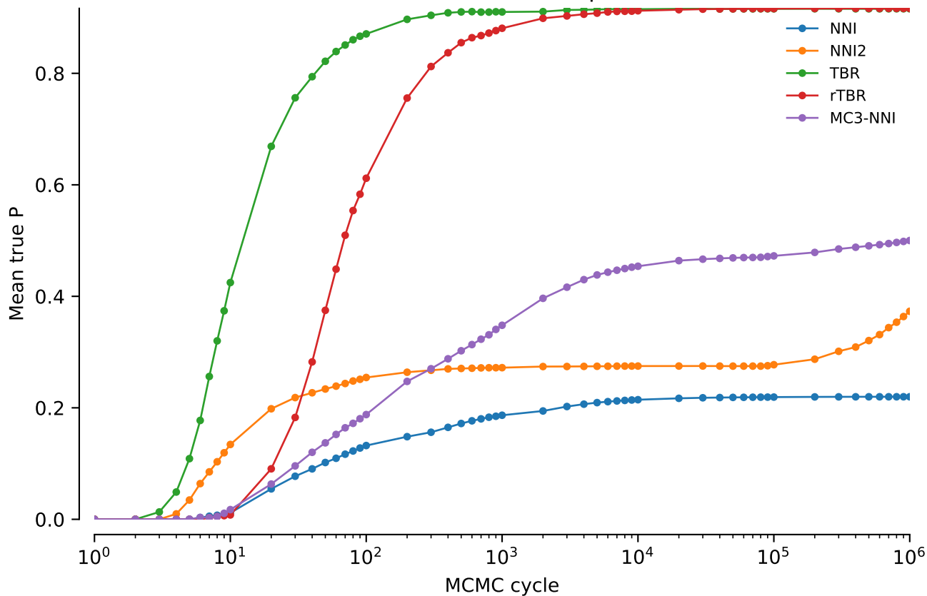
vert.nd6.tw5: Mean true P: power = 0.3
