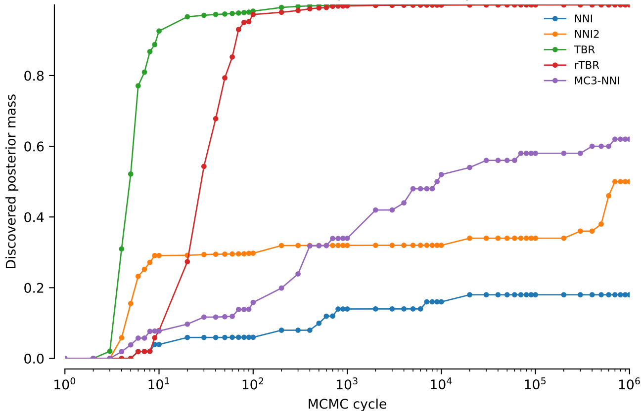
vert.nd6.tw5: Discovered posterior mass: power = 0.4
