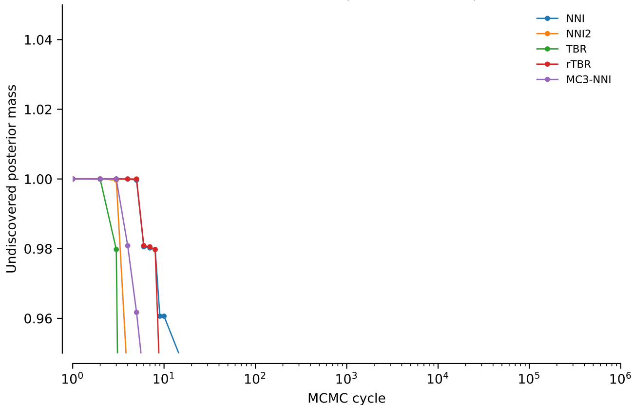
vert.nd6.tw5: Undiscovered posterior mass: power = 0.4
