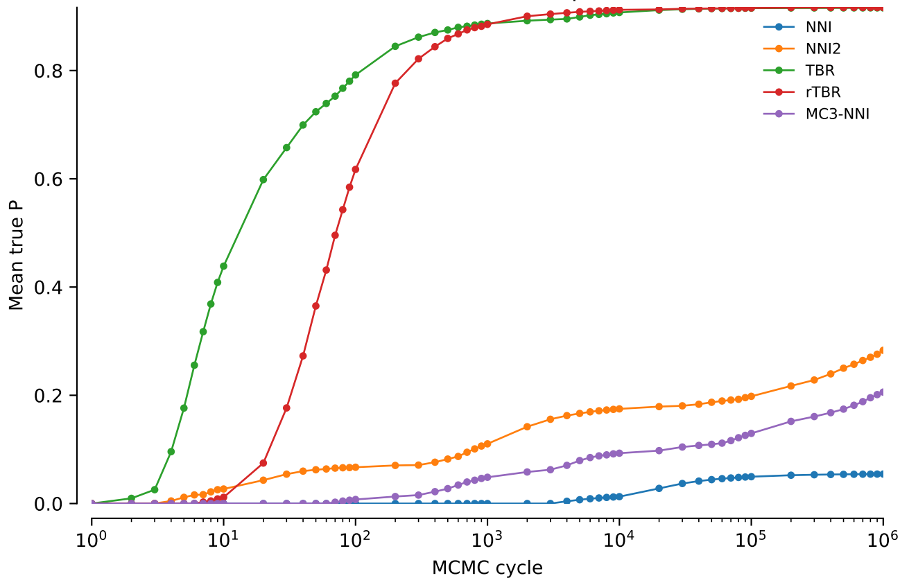
vert.nd6.tw5: Mean true P: power = 0.5
